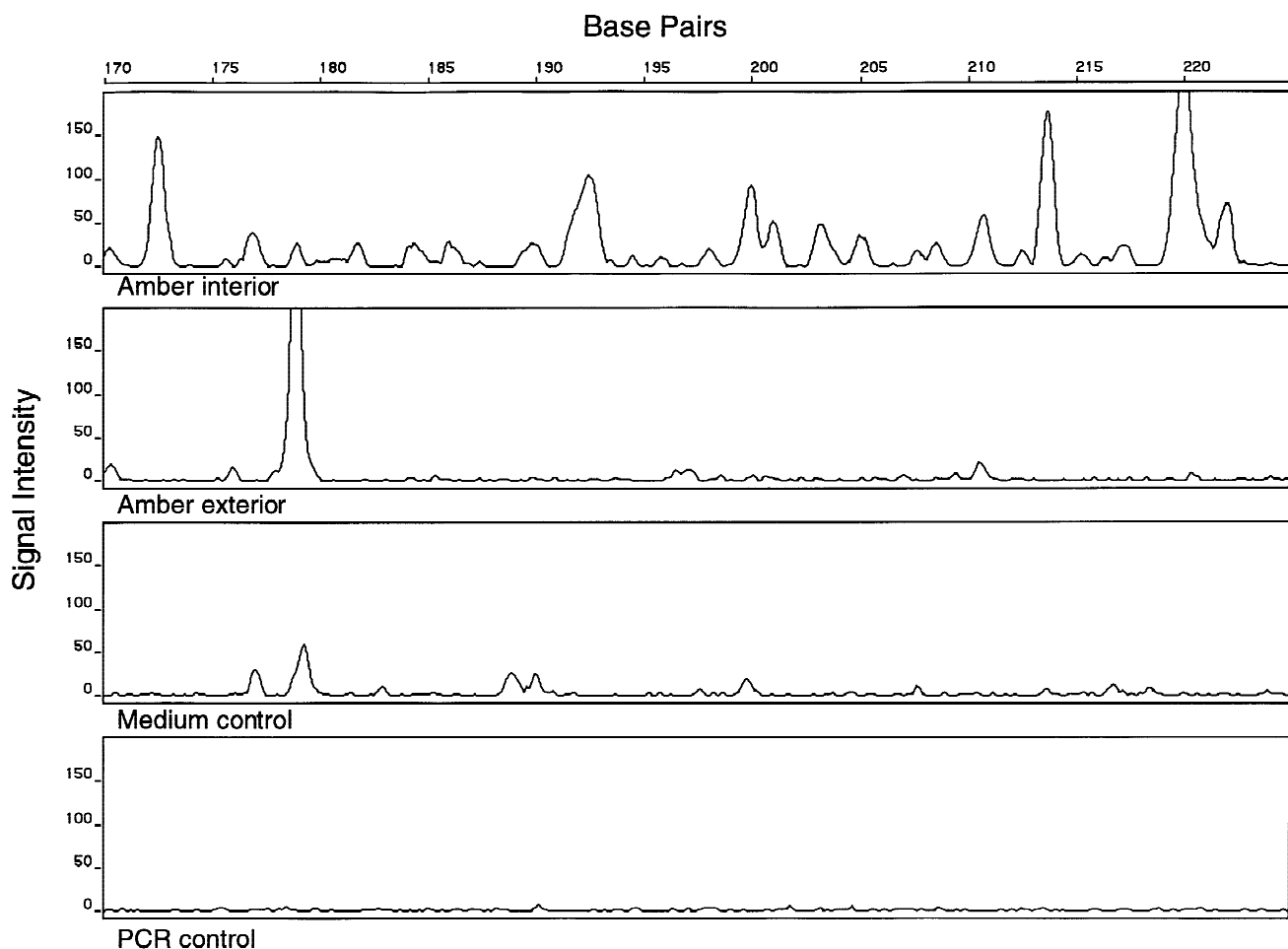
Fig. 3. Terminal restriction fragment (TRF) analysis of 16S 16S rRNA from amber community. TRF patterns of total 16S rDNA isolated from amber interior, amber exterior, reagents, and culture media were performed as described by Clement et al. [6]. DNA fragments 70–320 nucleotides (nt) in length resulting from SauIIIa digestion of amplified community 16S 16S rRNA are shown for one sample.
