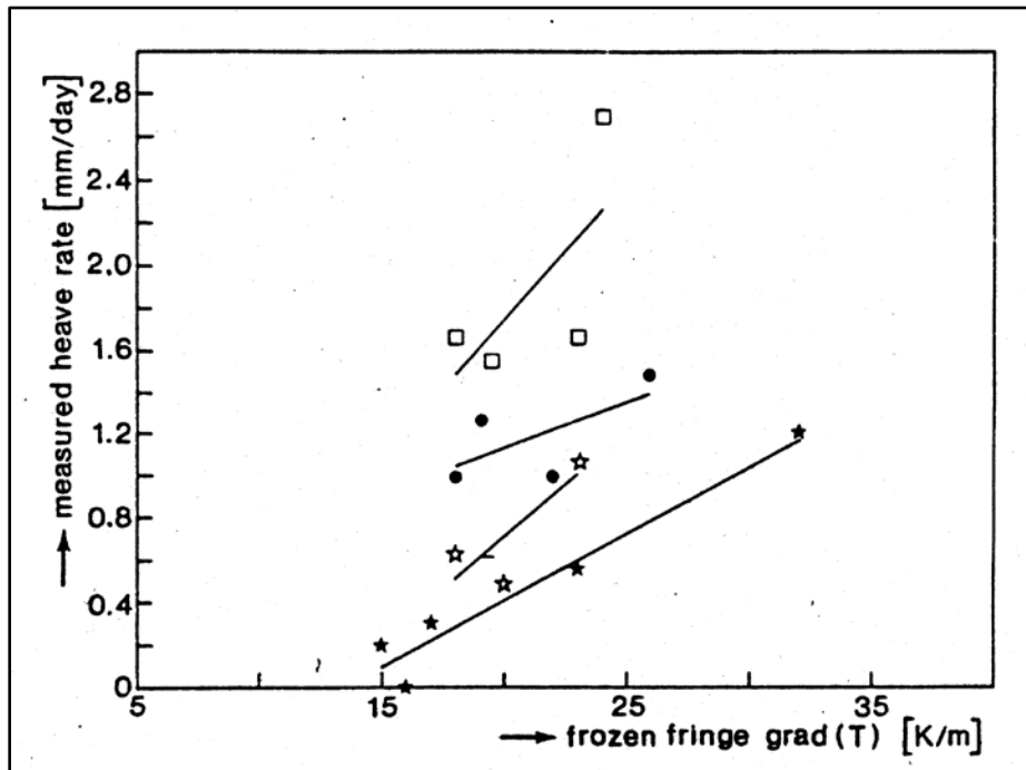
Figure B-4. Measured heave rates ( \text{mm day}^{-1} ) as a function of \text{Grad } T ( \text{K m}^{-1} ) in the frozen fringe for: loamy sand (solid circles); sandy loam (open squares); river basin clay (open stars); crushed concrete (solid stars). (after Van Loon, 1991).
