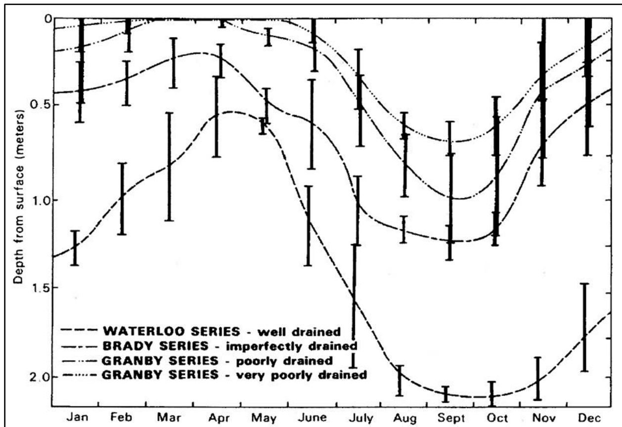
Figure Q-1. Average and seasonal variation in groundwater table levels in the Waterloo soil catena in southern Ontario during the period 1971-75 (after Mackintosh & van der Hulst, 1978).
