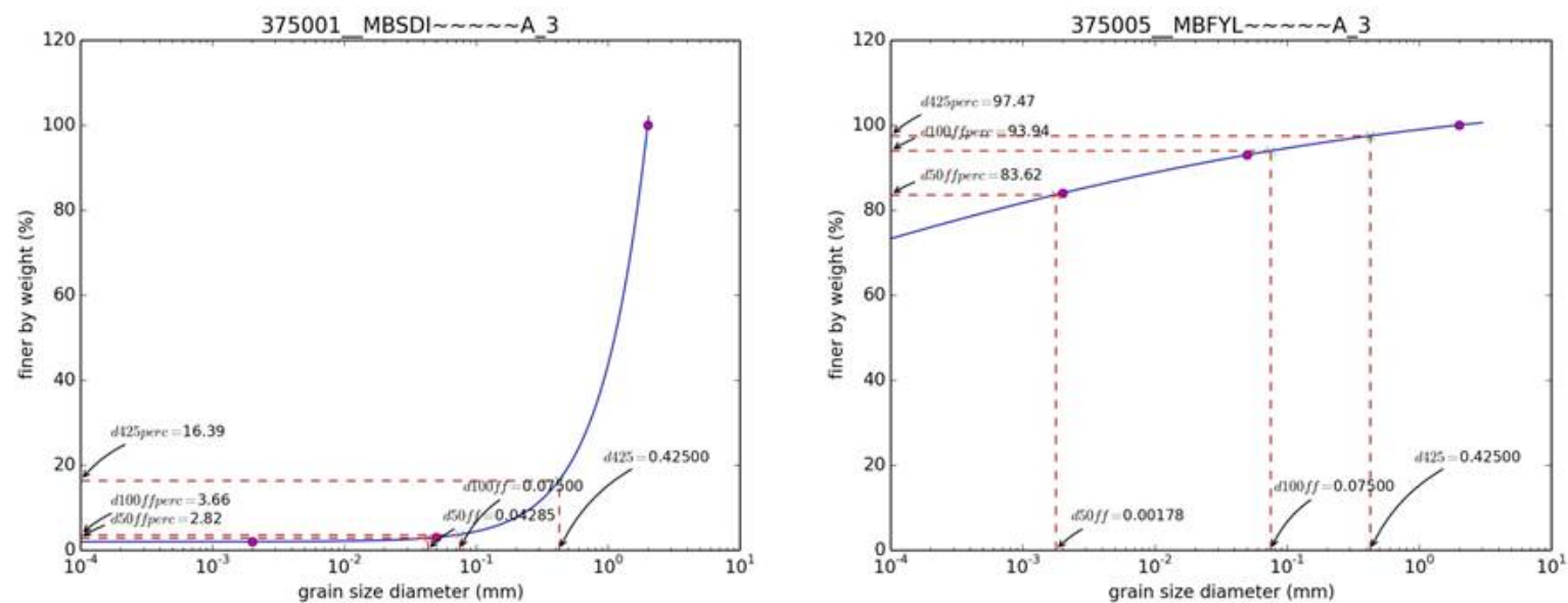
Figure P-3. Examples of automated PTF curve-fitting for estimating particle-size distribution parameters (Alberta and Manitoba soils).
