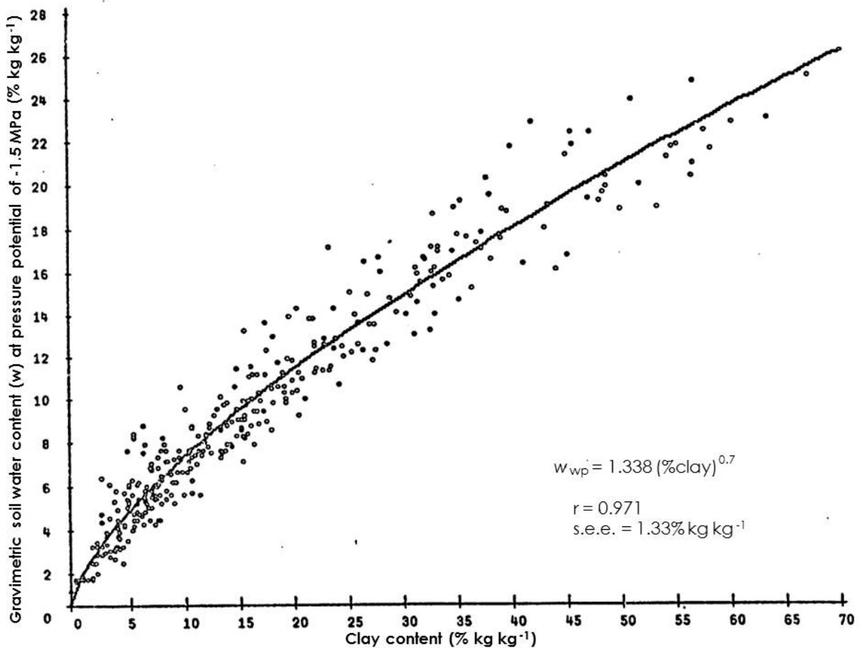
Figure L-2. Plot of the gravimetric soil water content at a pressure potential of -1.5 \text{ MPa} ( w_{wp} ) vs. clay content of Ontario soils. (after McBride & Mackintosh, 1984).
