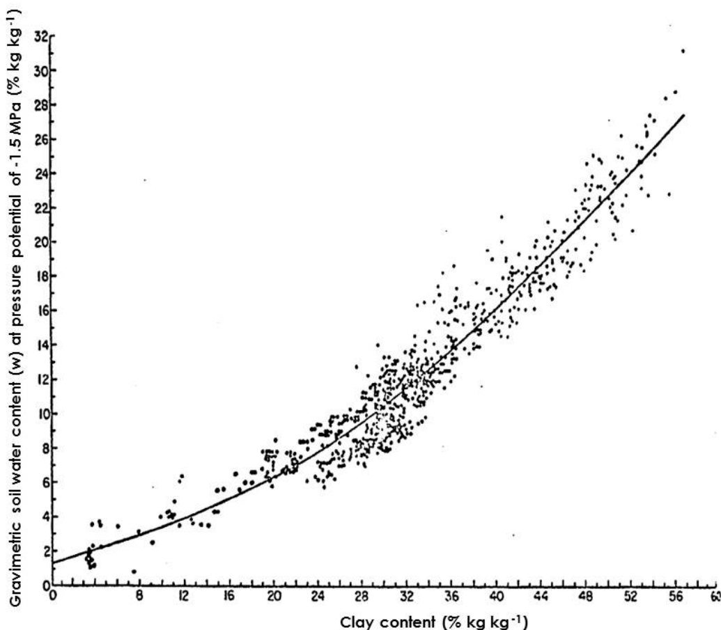
Figure L-3. Plot of the gravimetric soil water content at a pressure potential of -1.5MPa ( w_{wp} ) vs. clay content as determined by the hydrometer method for 730 Iowa soils. (after Nielsen & Shaw, 1958).
