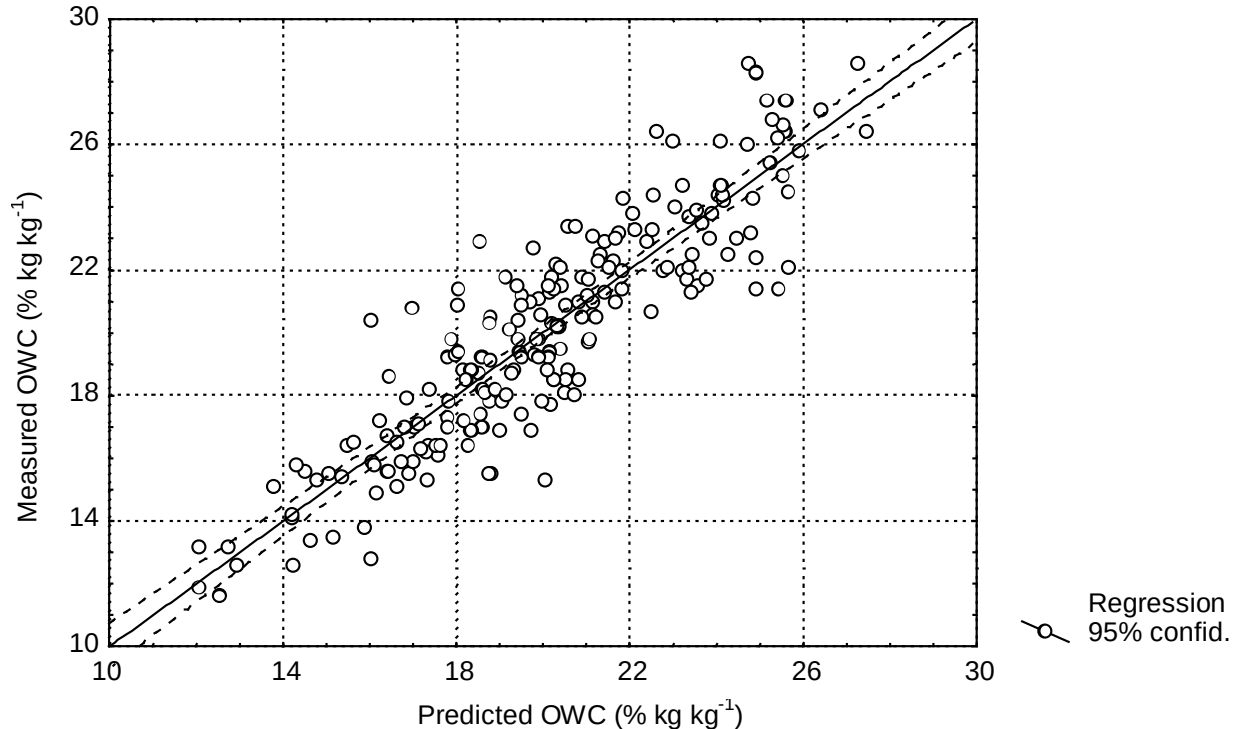
Figure N-5. Estimation of OWC based on linear effects for soil constituents (Eqn. N-2).
