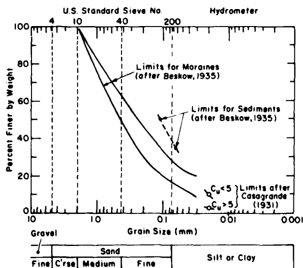
Figure 20. Grain size frost susceptibility criteria according to Riis (1948).
